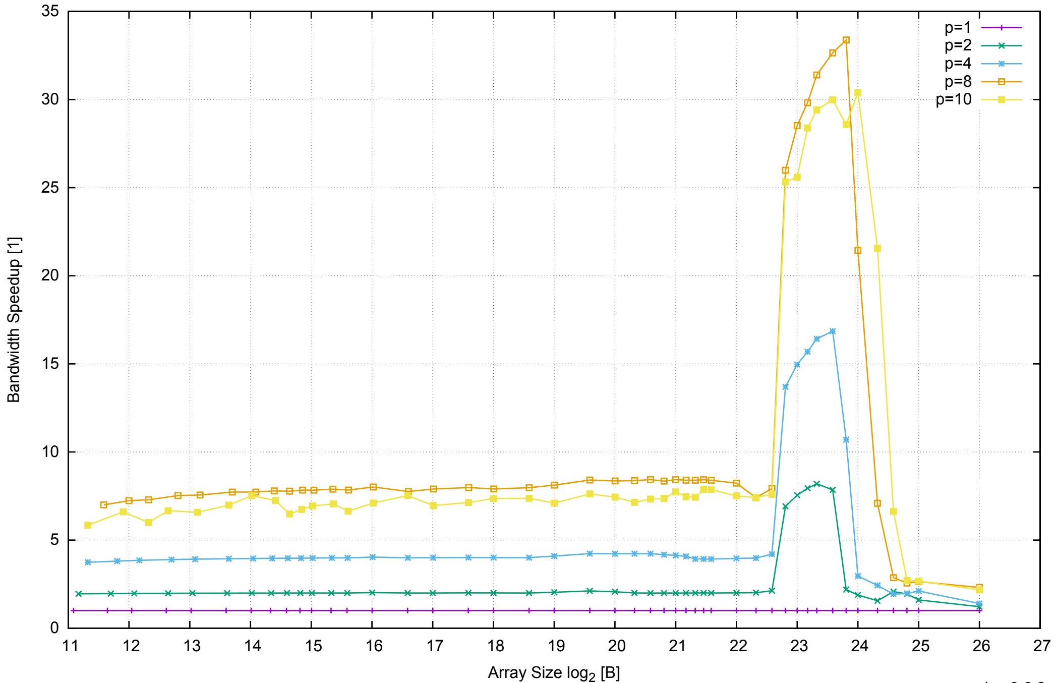
test-pilsner - Speedup of Memory Bandwidth - ScanWrite64PtrSimpleLoop
