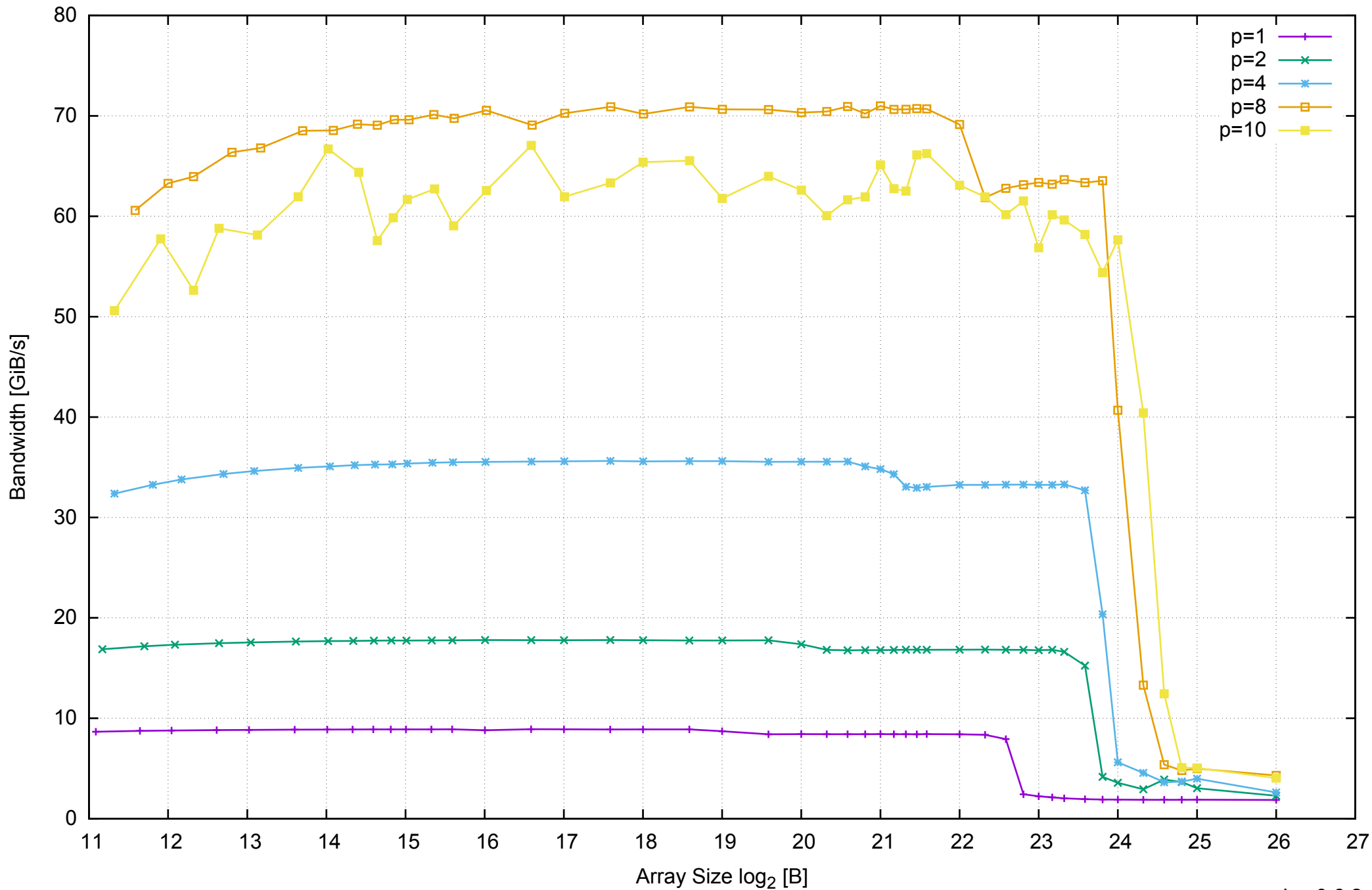
test-pilsner - Memory Bandwidth - ScanWrite64PtrSimpleLoop
