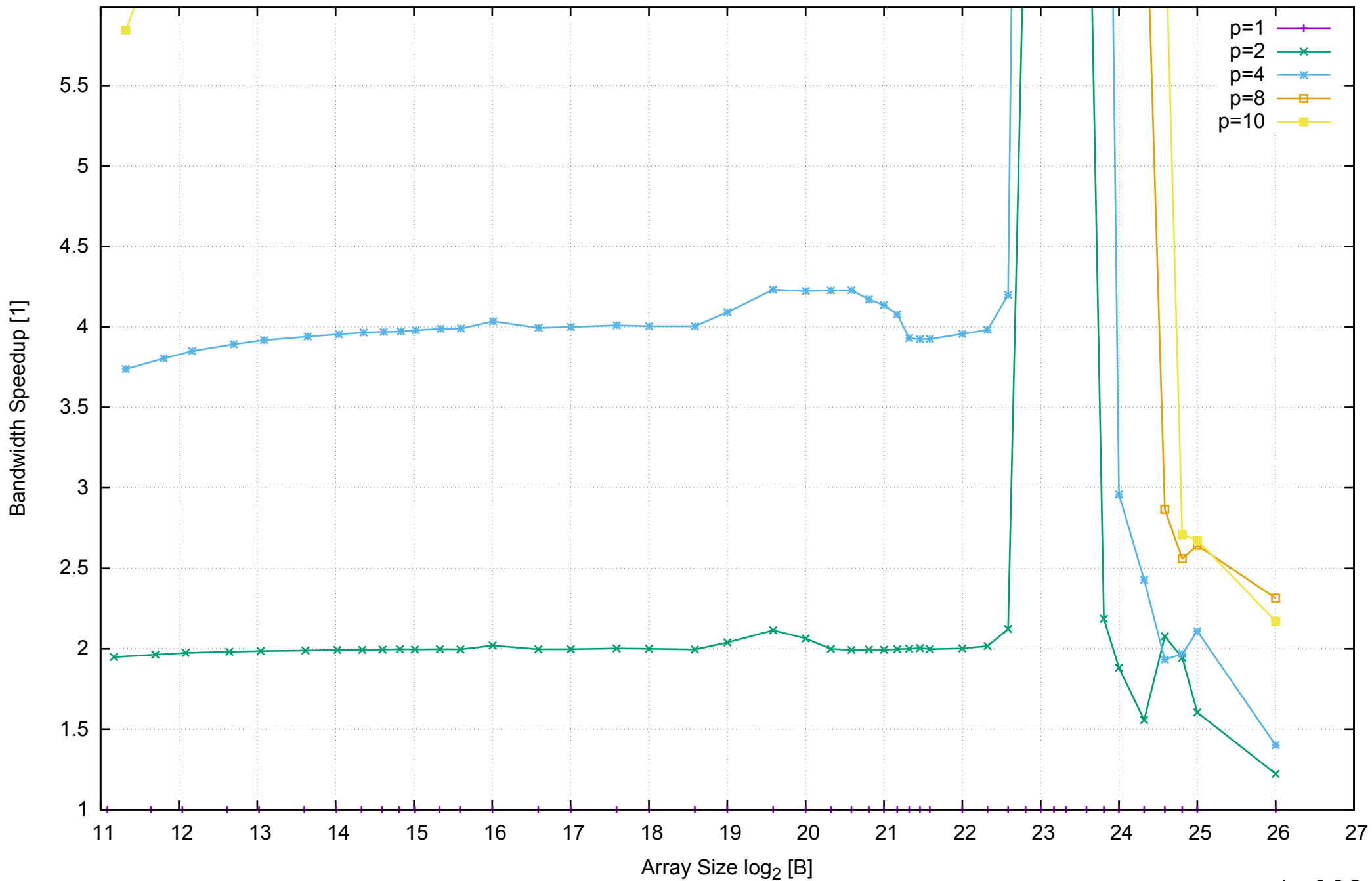
test-pilsner - Speedup of Memory Bandwidth (enlarged) - ScanWrite64PtrSimpleLoop
