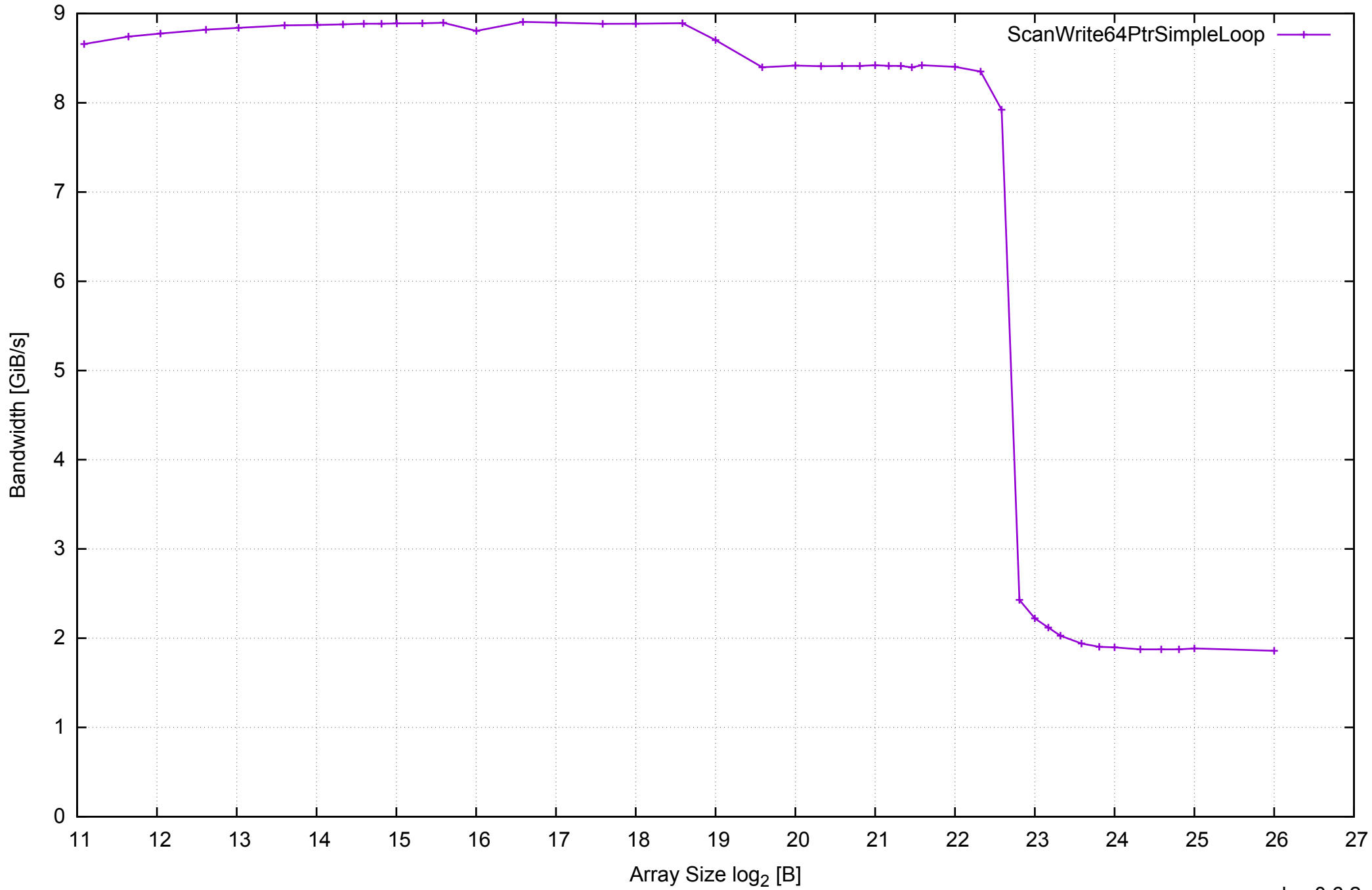
test-pilsner - One Thread Memory Bandwidth
