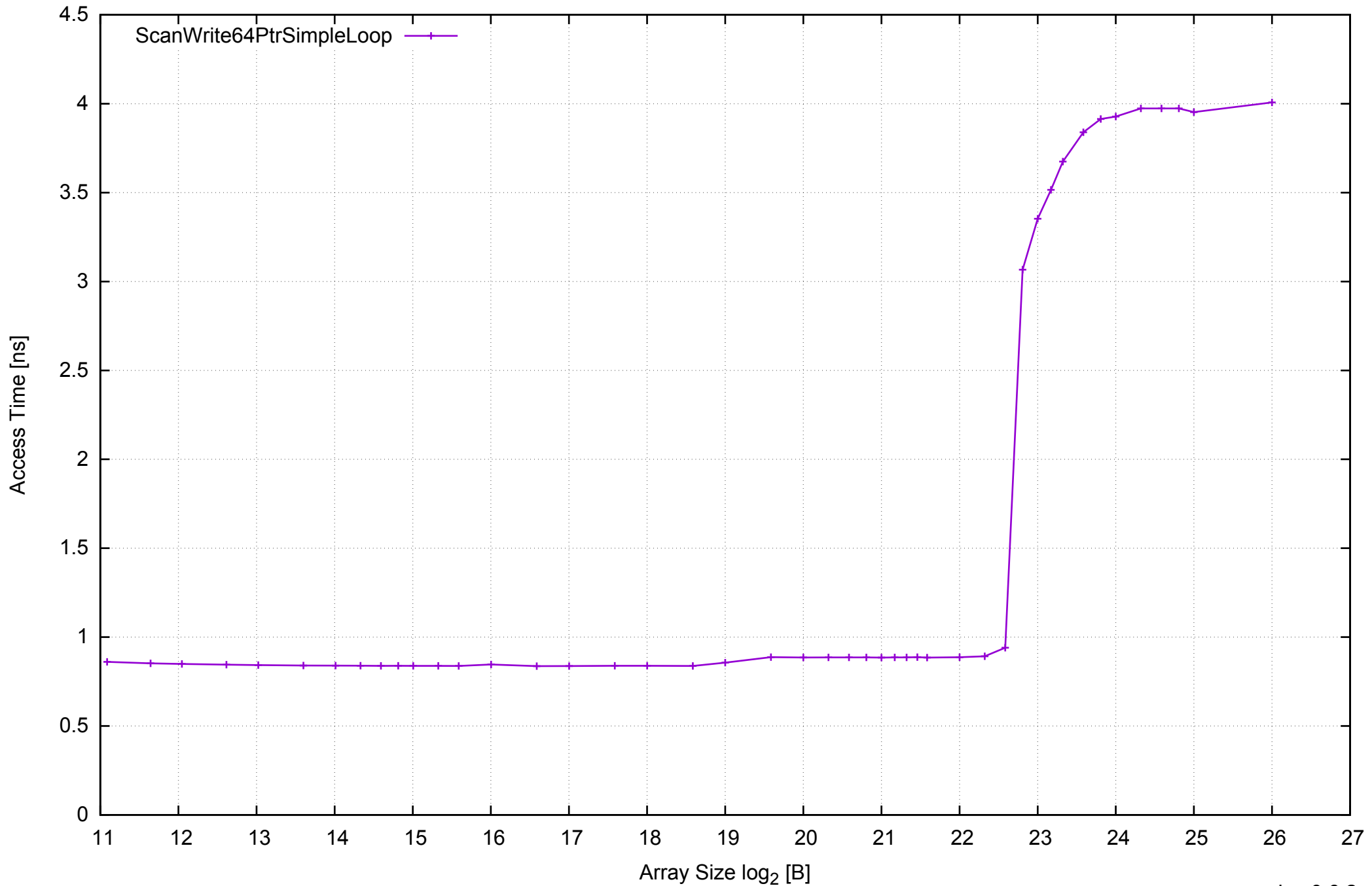
test-pilsner - One Thread Memory Latency
