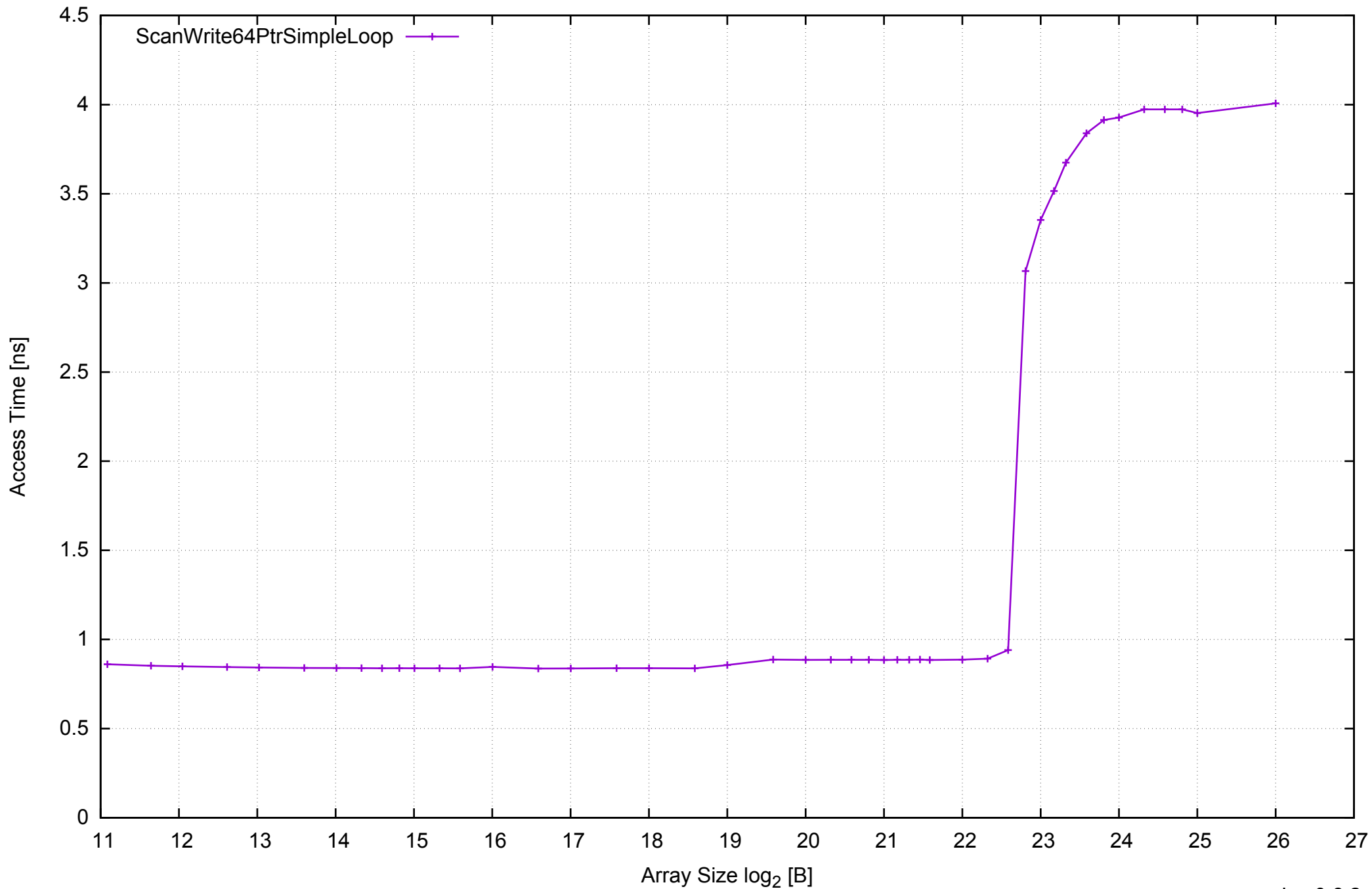
test-pilsner - One Thread Memory Latency (excluding Permutation)
