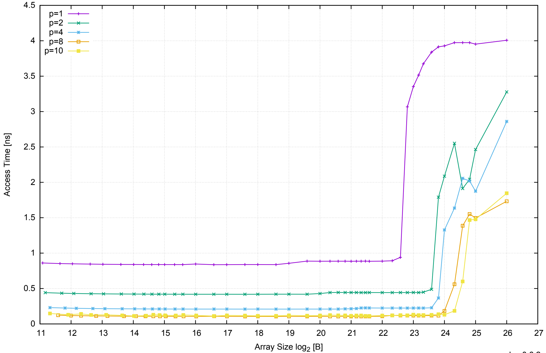
test-pilsner - Memory Latency - ScanWrite64PtrSimpleLoop
