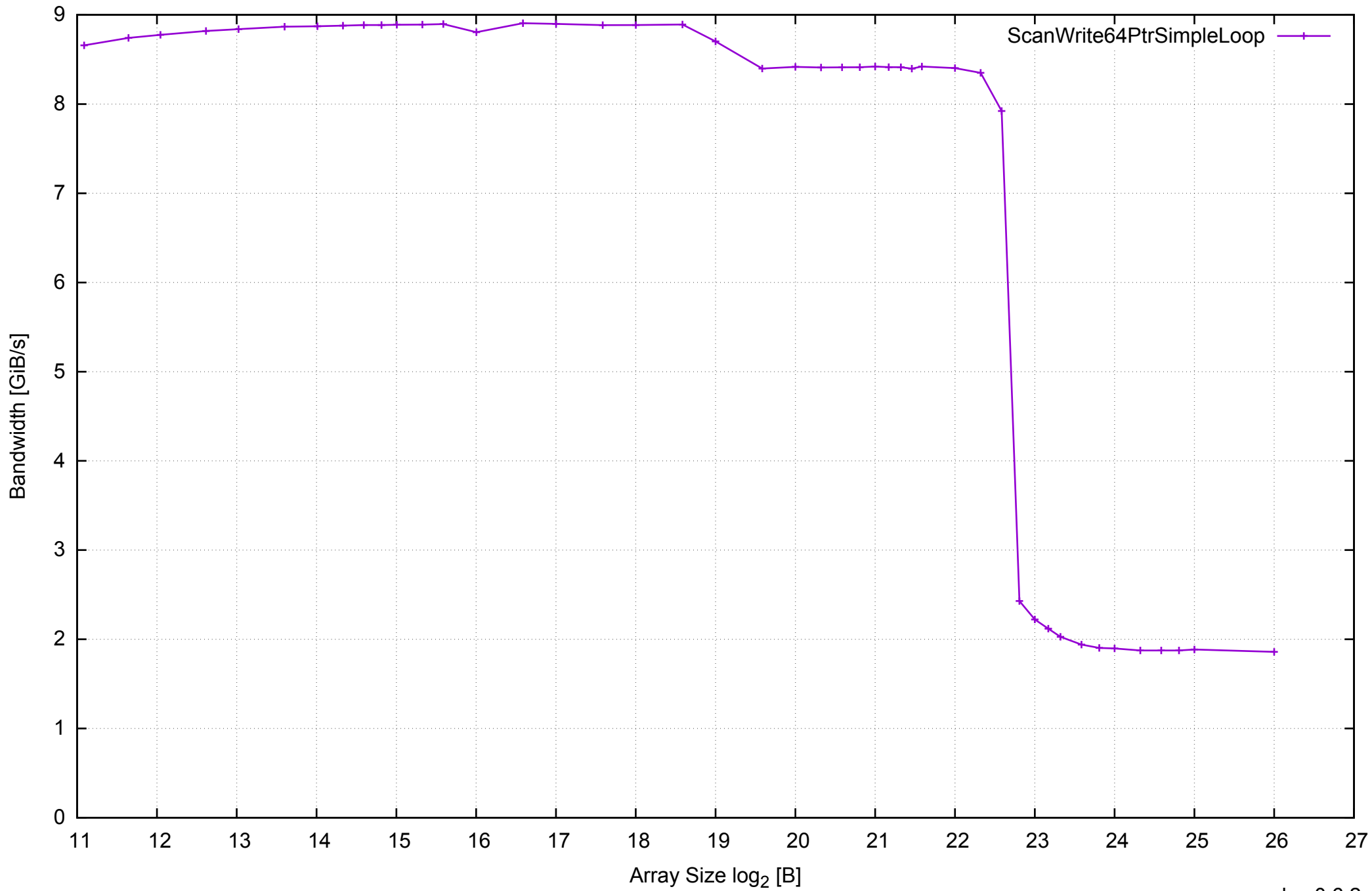
test-pilsner - One Thread Memory Bandwidth (only 64-bit Reads)
