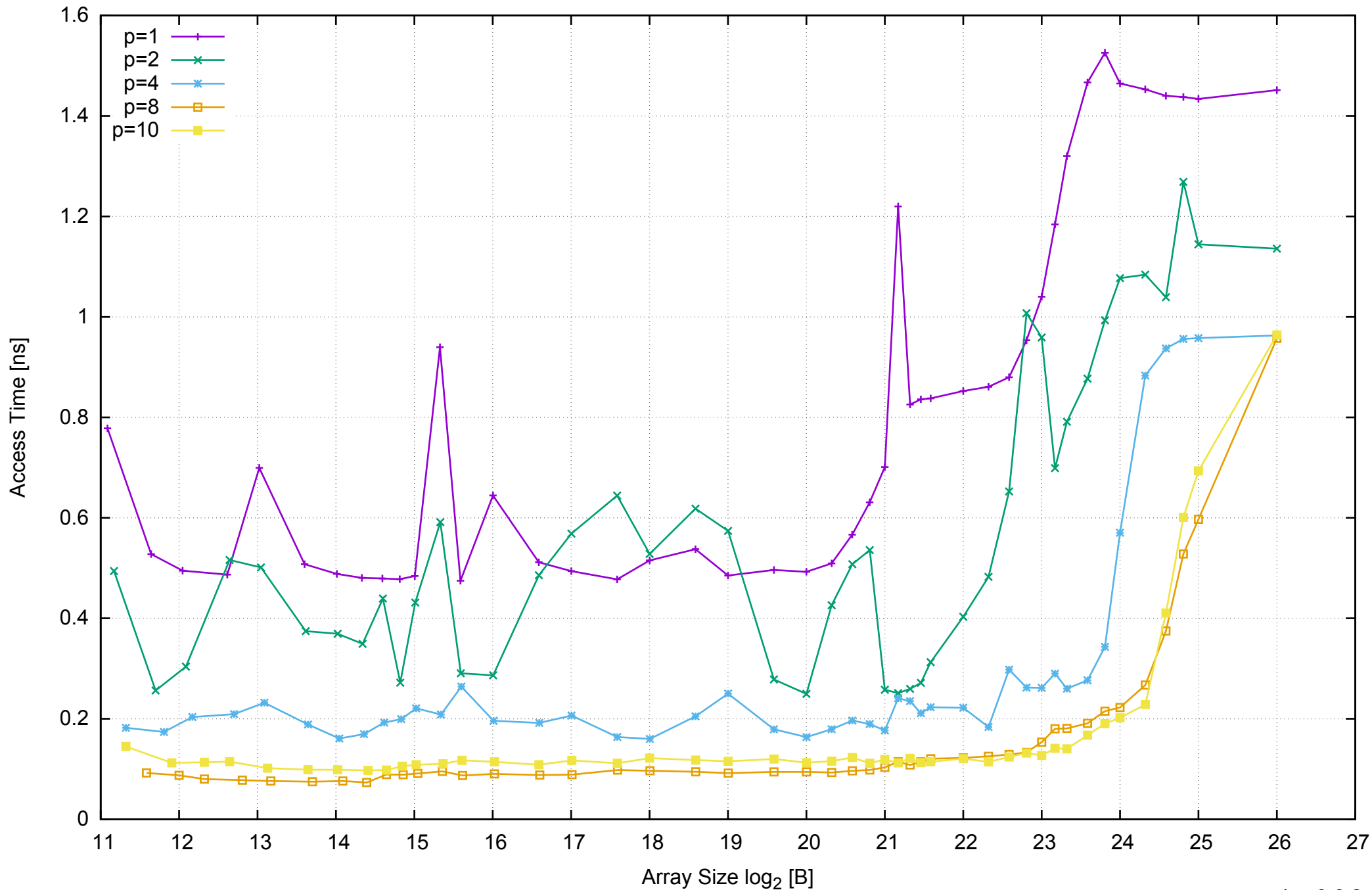
test-carpaccio - Memory Latency - ScanWrite64PtrSimpleLoop
