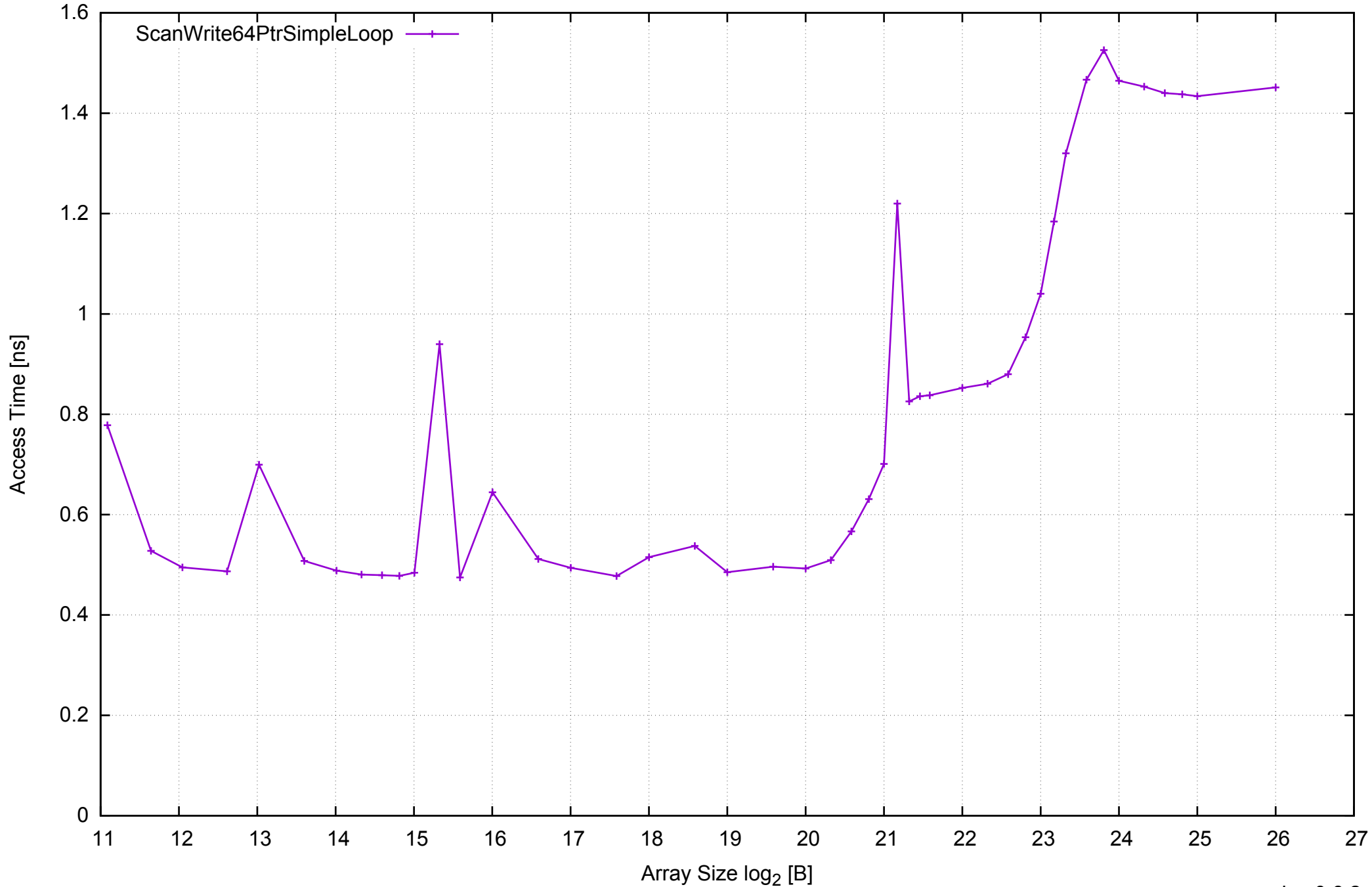
test-carpaccio - One Thread Memory Latency (excluding Permutation)
