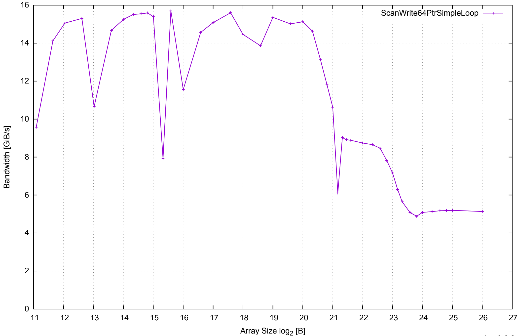
test-carpaccio - One Thread Memory Bandwidth
