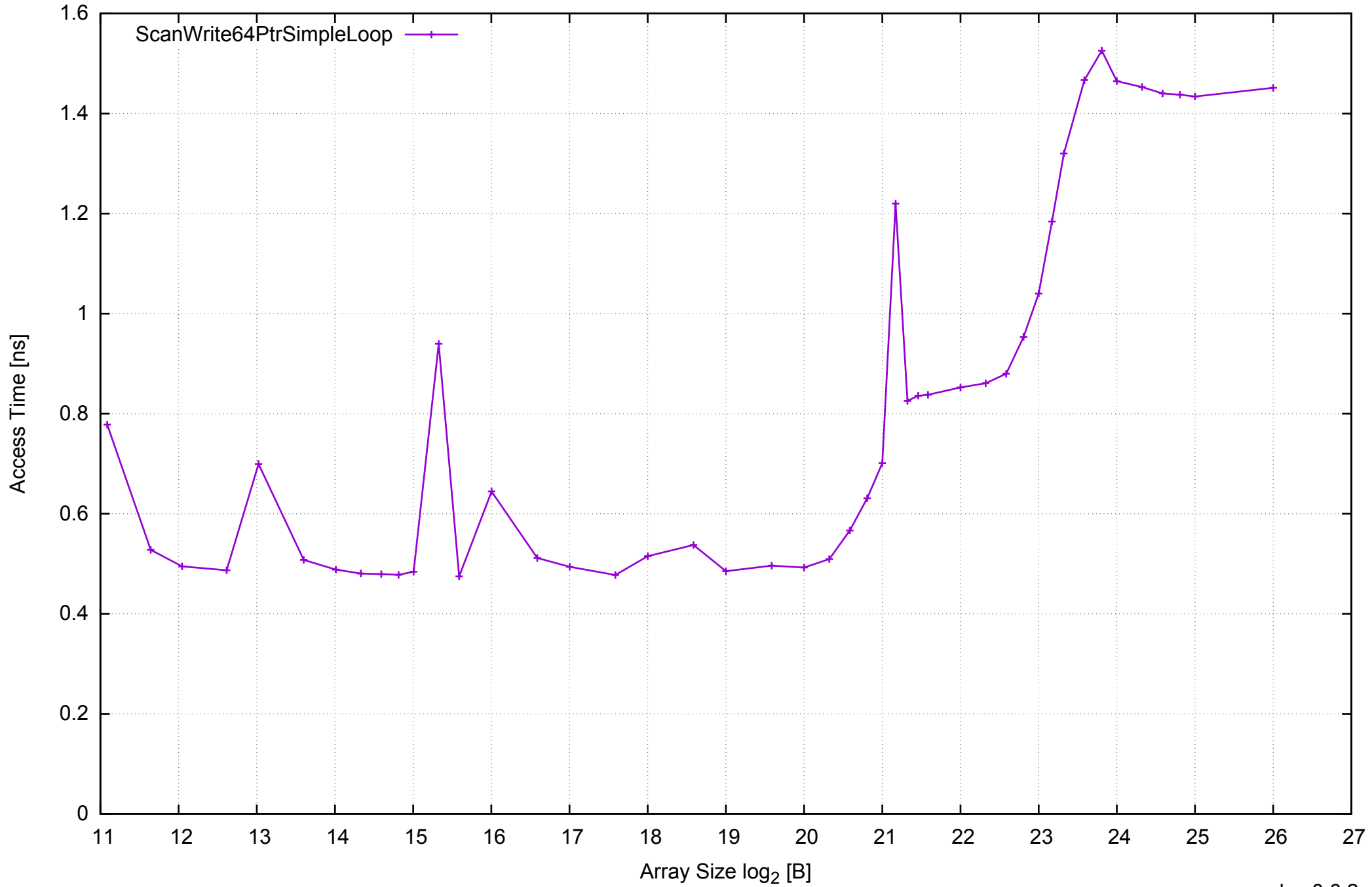
test-carpaccio - One Thread Memory Latency
