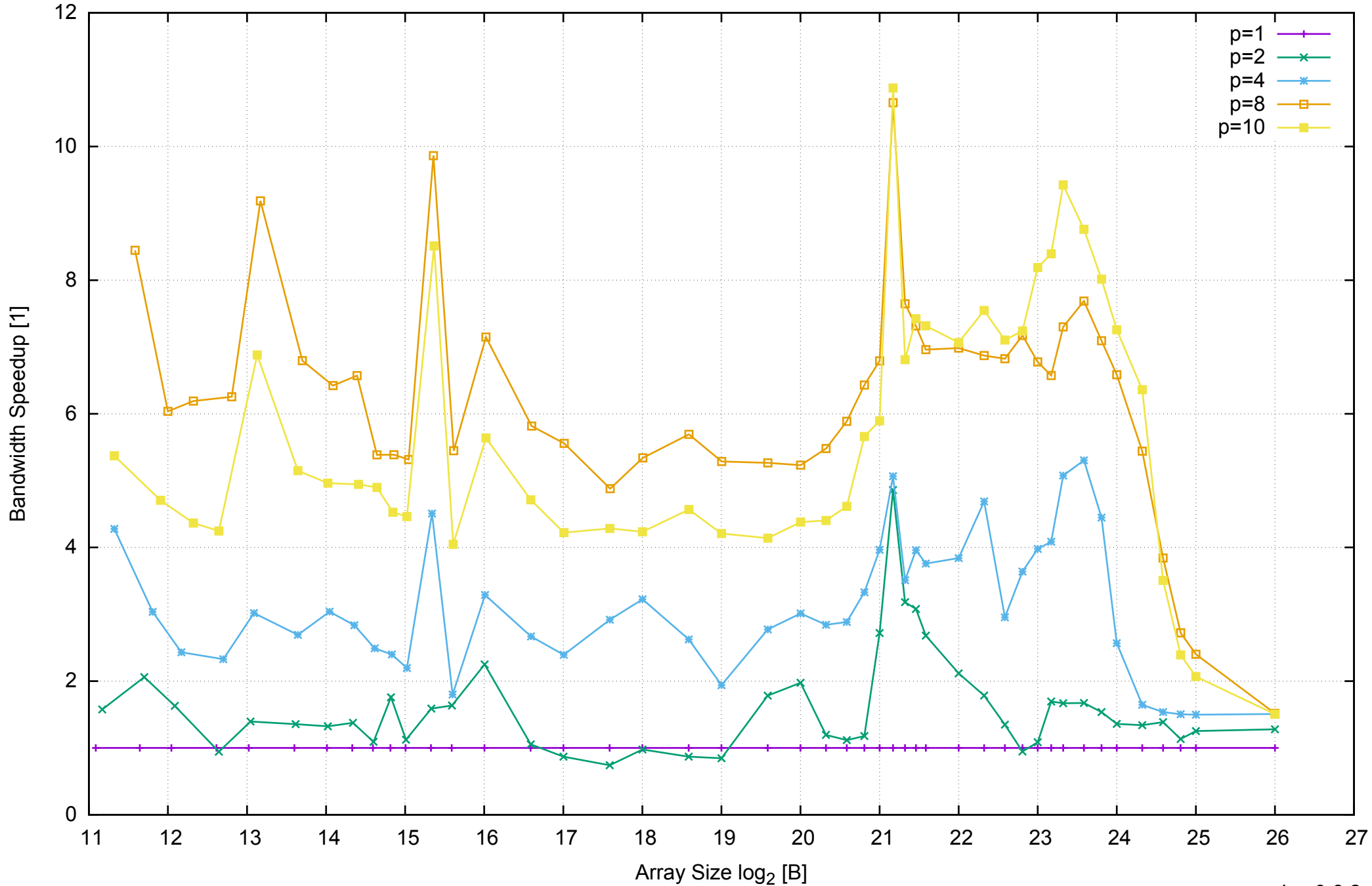
test-carpaccio - Speedup of Memory Bandwidth - ScanWrite64PtrSimpleLoop
