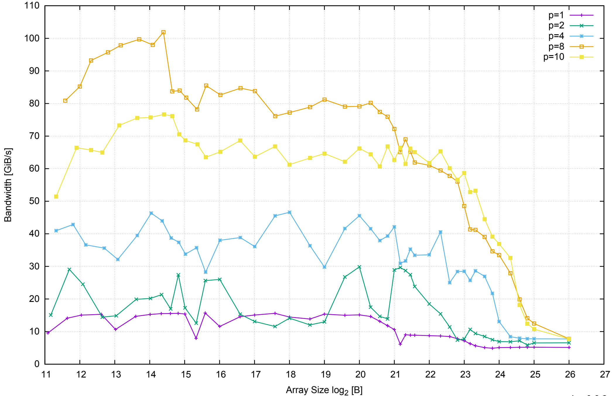
test-carpaccio - Memory Bandwidth - ScanWrite64PtrSimpleLoop
