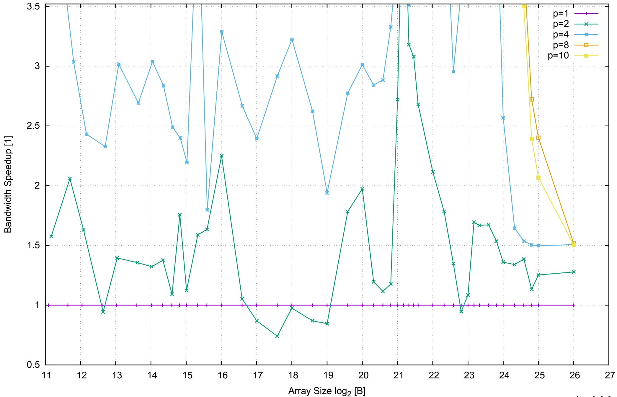
test-carpaccio - Speedup of Memory Bandwidth (enlarged) - ScanWrite64PtrSimpleLoop
