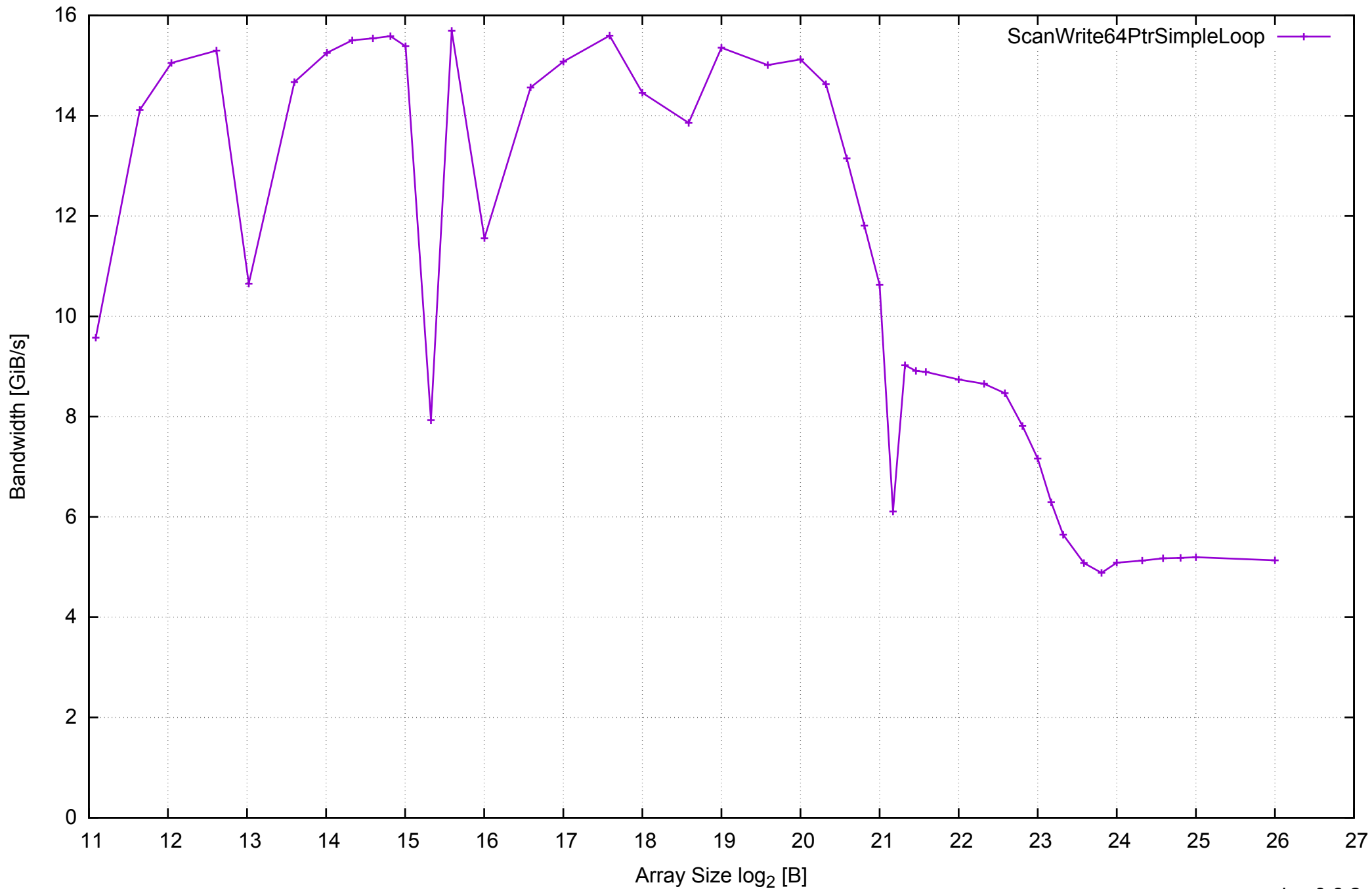
test-carpaccio - One Thread Memory Bandwidth (only 64-bit Reads)
